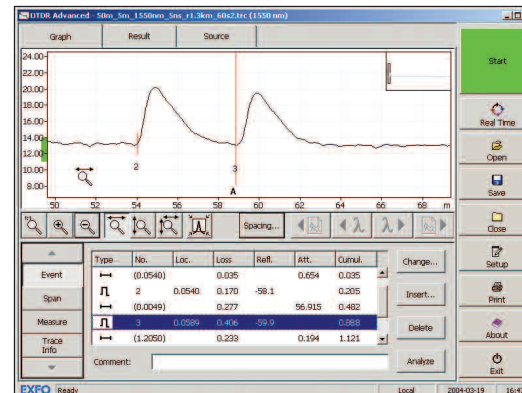
The FTB-7000E OTDR's market-leading dead zone enables the full characterization of a typical tie-cable—as short as 4.5 m with UPC connectors (reflectance below -45 dB).
