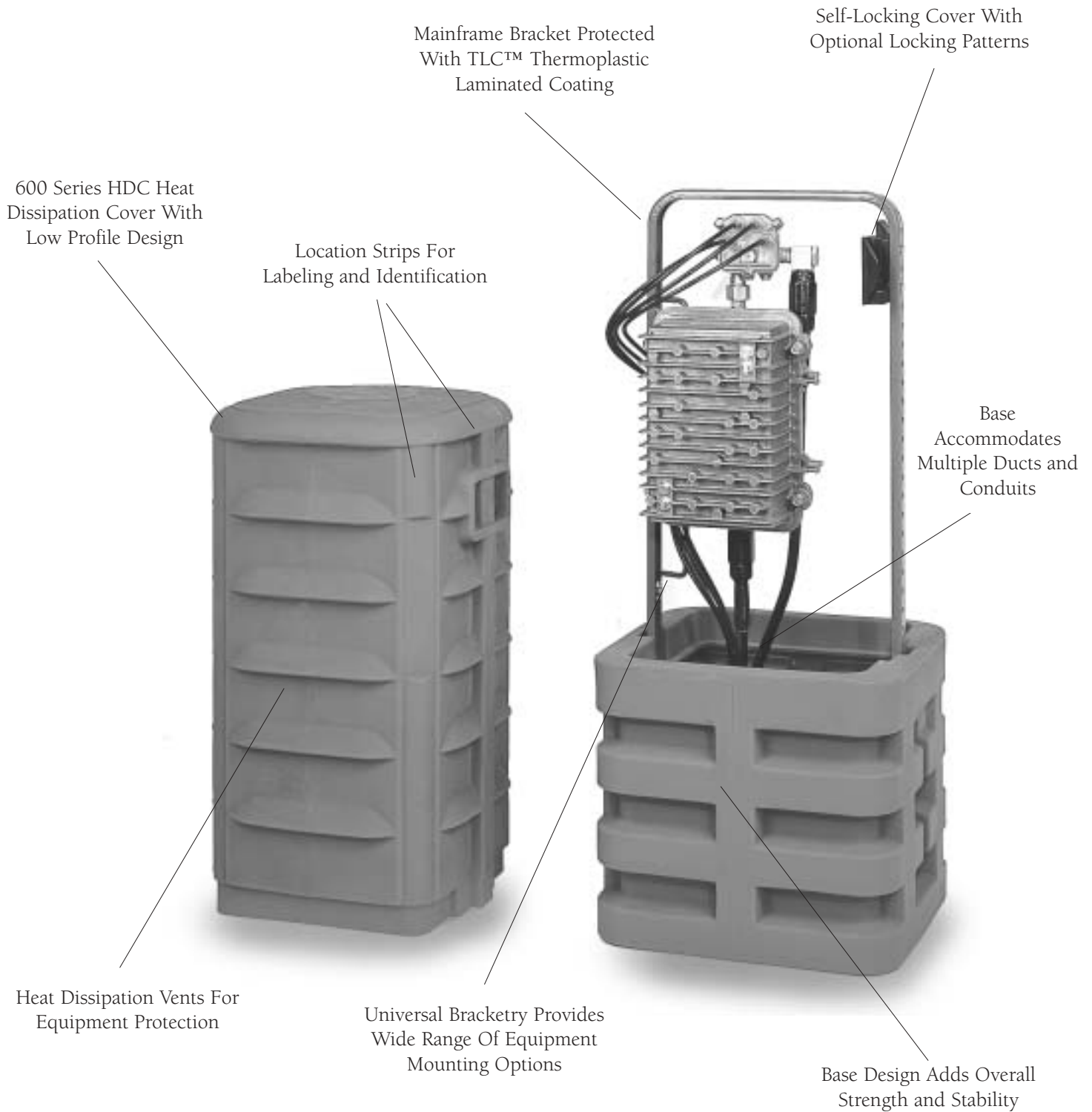
SPH12123 Low Profile Pedestal
