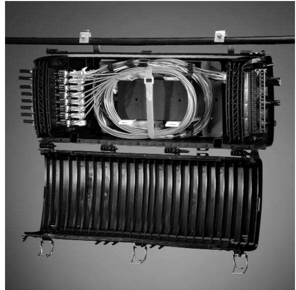
OptiSheath Classic Aerial Terminal (open) | Photo SHD168
