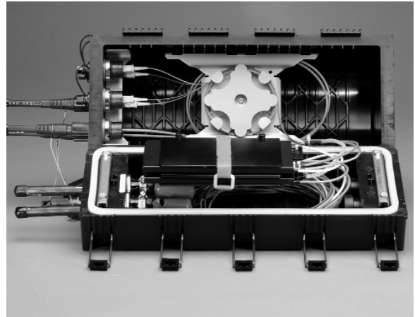
OptiSheath Advantage Sealed Terminal, (open) | Photo SHD160
