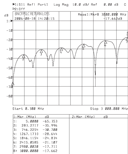
BNCFSLC Return Loss
